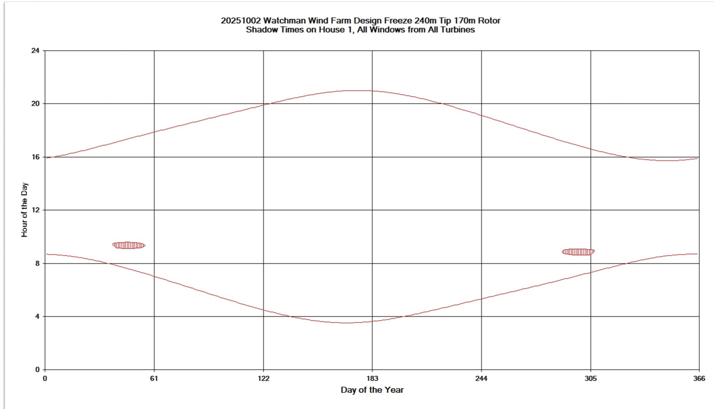
Figure 12.1.1: Potential Shadow Flicker Effect at H1
