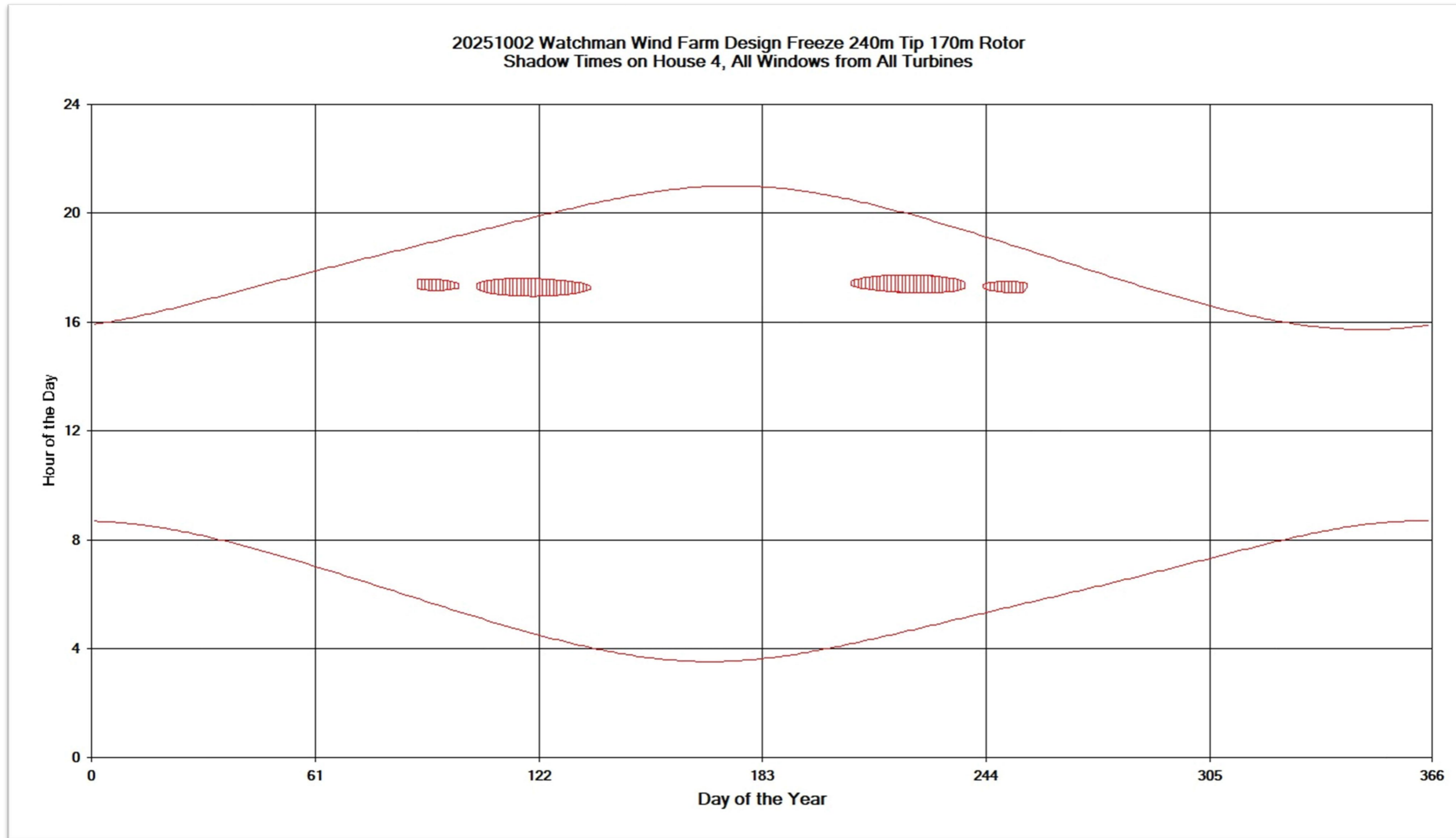
Figure 12.1.4: Potential Shadow Flicker Effect at H4
