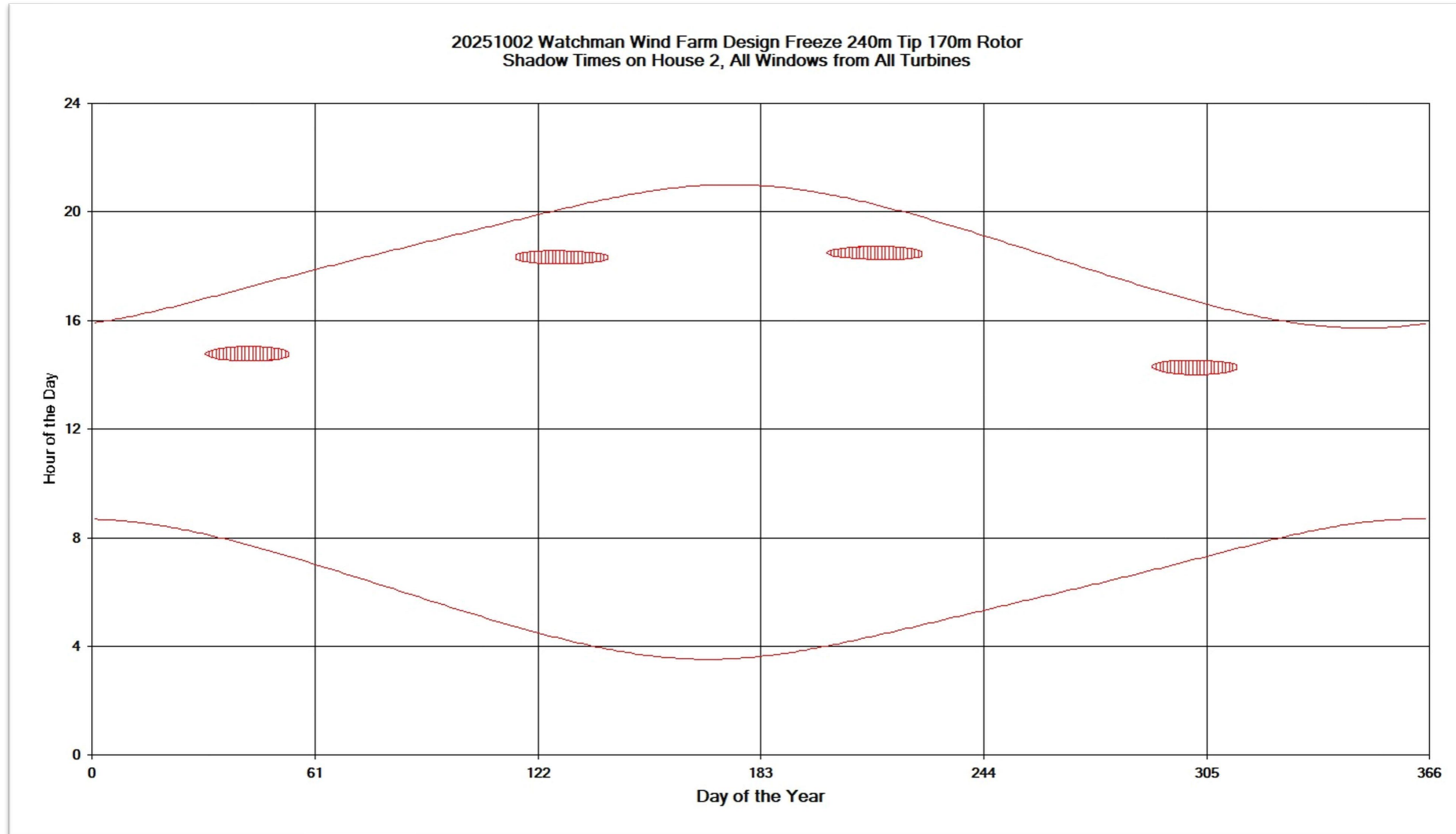
Figure 12.1.2: Potential Shadow Flicker Effect at H2
