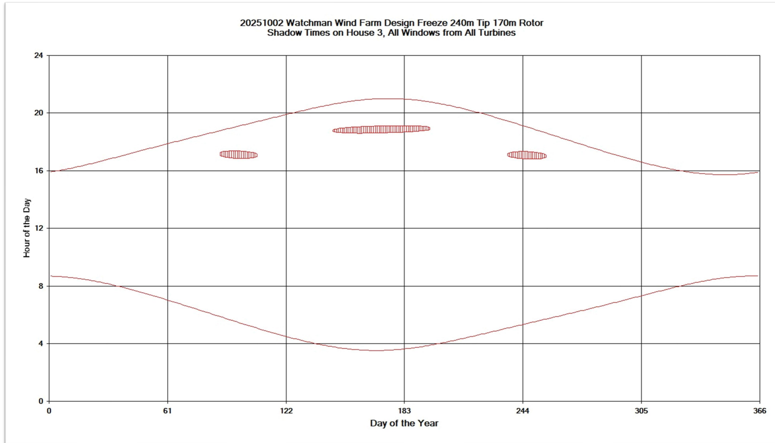
Figure 12.1.3: Potential Shadow Flicker Effect at H3
